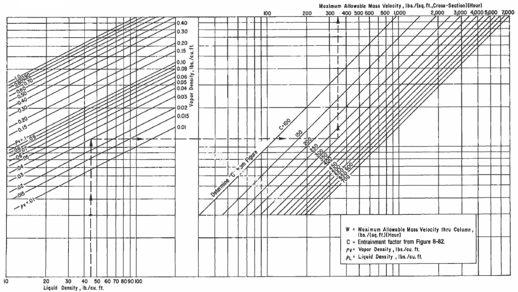
Figure 8-83. Allowable mass velocity for fractionation, absorption, and stripping columns.
